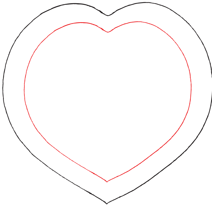
4.25" x 4" Heart Template Imprint Area: 3" x 2½" (3/8" from edge) Minimum Font Size: 9 point
